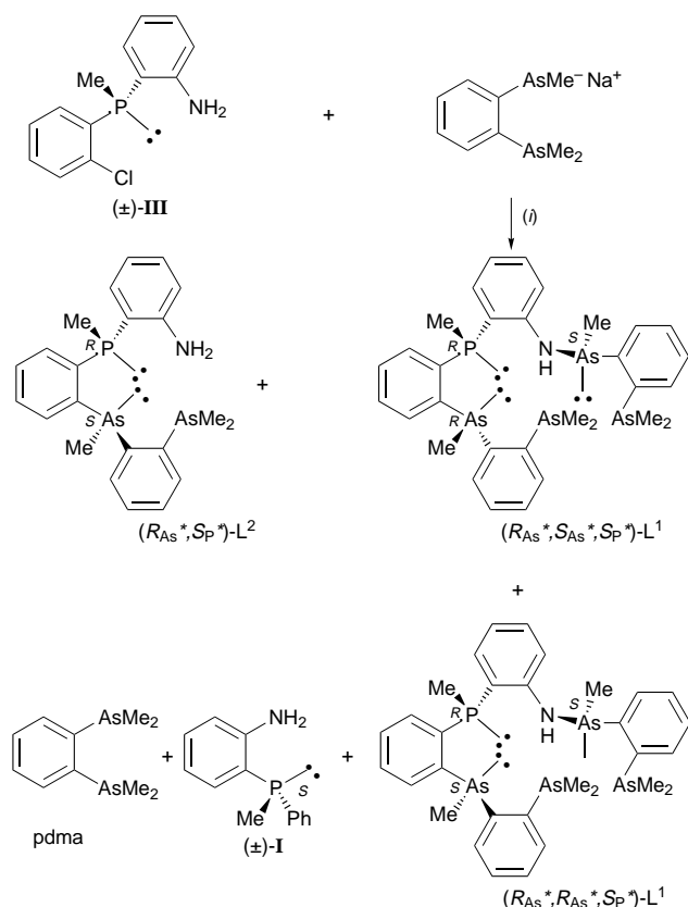
Scheme 4 Only one enantiomer of the chiral compounds is shown. (i) thf, –78 °C
