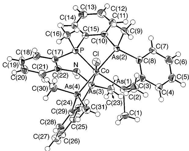
Fig. 3 Molecular structure of the cation [\text{CoCl}\{(R_{\text{As}}^*, S_{\text{As}}^*, S_{\text{P}}^*)\text{-L}^1\}]^{2+}
