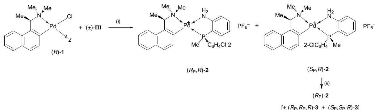
Scheme 2 (i) \text{MeOH} , \text{NH}_4\text{PF}_6 in water; (ii) (R_p^*,R_p^*)\text{-C}_6\text{H}_4(\text{PMePh})_2 -1,2 in \text{CH}_2\text{Cl}_2
