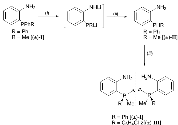
Scheme 1 (i) 3Li in thf; (ii) water; (iii) Na in thf; MeI or \text{C}_6\text{H}_4\text{Cl}_2\text{-1,2} in thf
